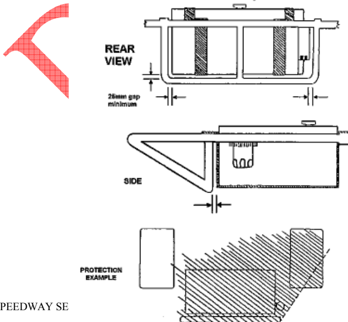
Fig 18 FUEL TANK PROTECTOR
