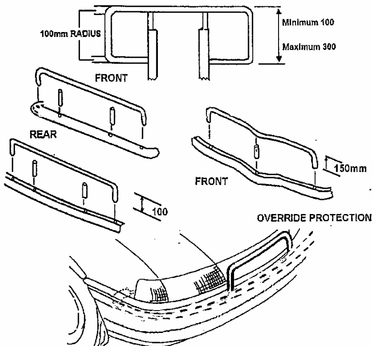
Fig 15 Front & Rear Override Bars
