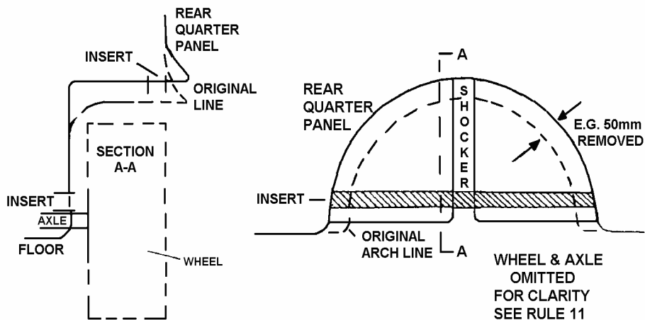
Fig 7 Wheel Arch Modification
